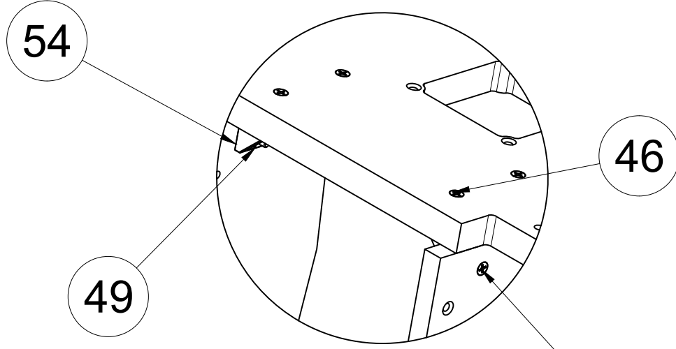
DETAIL E SCALE 1:3
